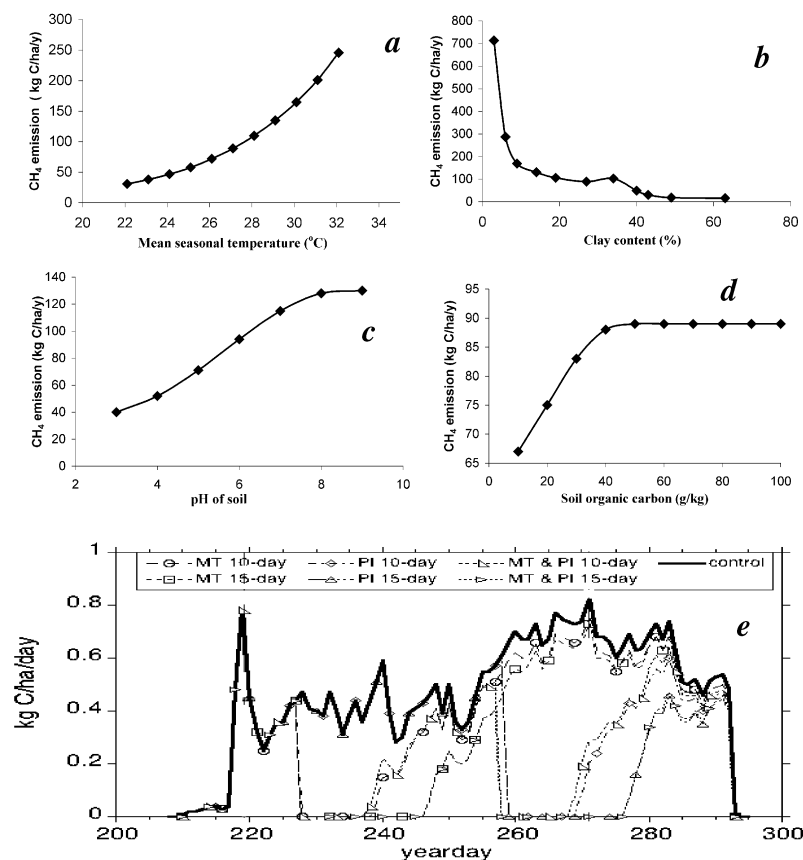
Figure 3. Sensitivity of DNDC simulated annual \text{CH}_4 flux from a Cuttack paddy field with (a) mean seasonal temperature, (b) soil texture, (c) soil pH, (d) soil organic C content and (e) water management. MT, Maximum tillering stage; PI, Panicle stage.
