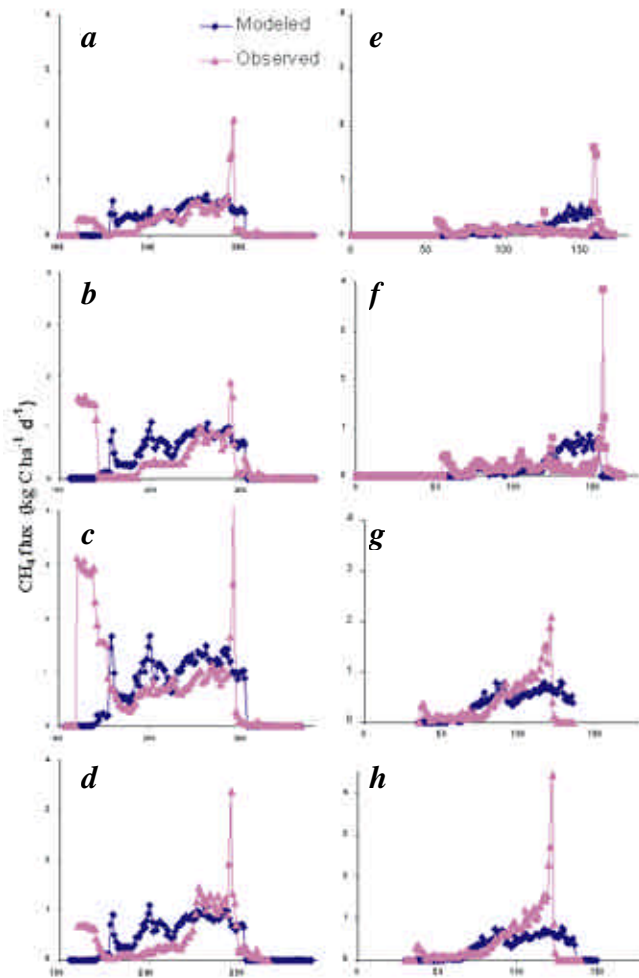
Figure 1. Modelled and measured daily methane emissions at eight sites with continuous flux measurements 26 . All the sites were continuously flooded. Four of the sites were measured in the kharif season of 1996; their treatments were (a) urea, (b) urea + compost, (c) urea + Sesbania (green manure) and (d) urea + Azolla (green manure). Two of the sites were measured in the rabi season of 1997; their treatments were (e) urea and (f) urea + rice straw. Two of the sites were measured in the rabi season of 1999; they had the same treatment (urea) but used different rice varieties: Ratna (g) and Lalat (h). DNDC simulations did not discriminate between these varieties.
