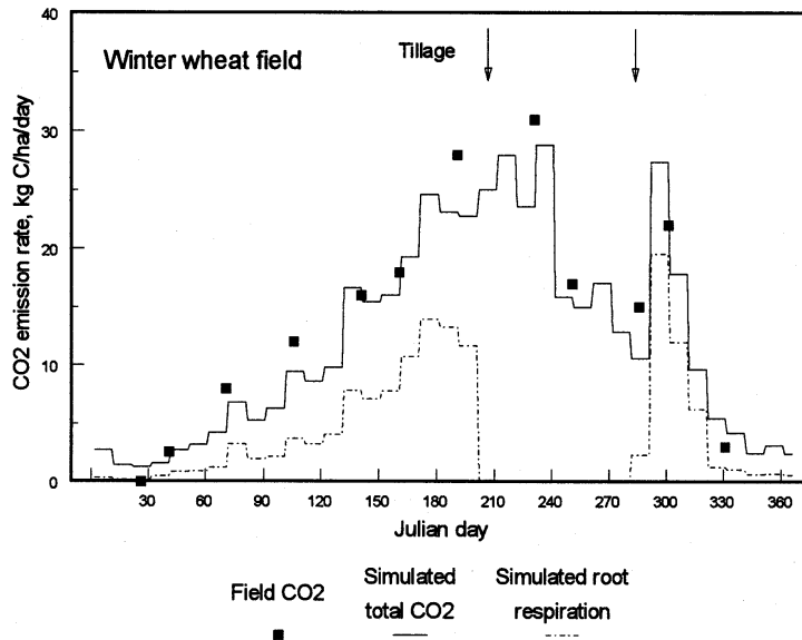
Figure 6. Comparison of simulated results and field data [Buyanovsky et al., 1986] on CO 2 emissions from a silty loam soil in a tilled and fertilized winter wheat field in Columbia, Missouri. After the winter wheat was planted in October, CO 2 emission rates increased due to tillage and root respiration of the young plants. Root respiration accounted for 30-70% of the CO 2 flux.
